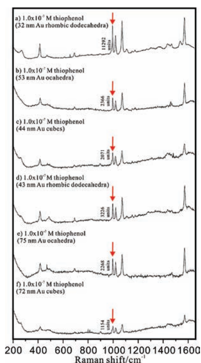
Figure 3. SERS spectra of 1.0 \times 10^{-7} M thiophenol in the cubic, octahedral, and rhombic dodecahedral Au nanocrystal solutions. Intensity of the band at 998 \text{ cm}^{-1} is given for each sample. This band is used for all SERS comparison purposes in this work. The excitation wavelength is 632.8 nm.
